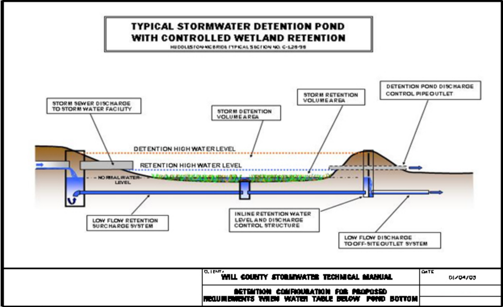
FIGURE 12 Detention Configuration for Proposed Requirements When Water Table is Below Pond Bottom
