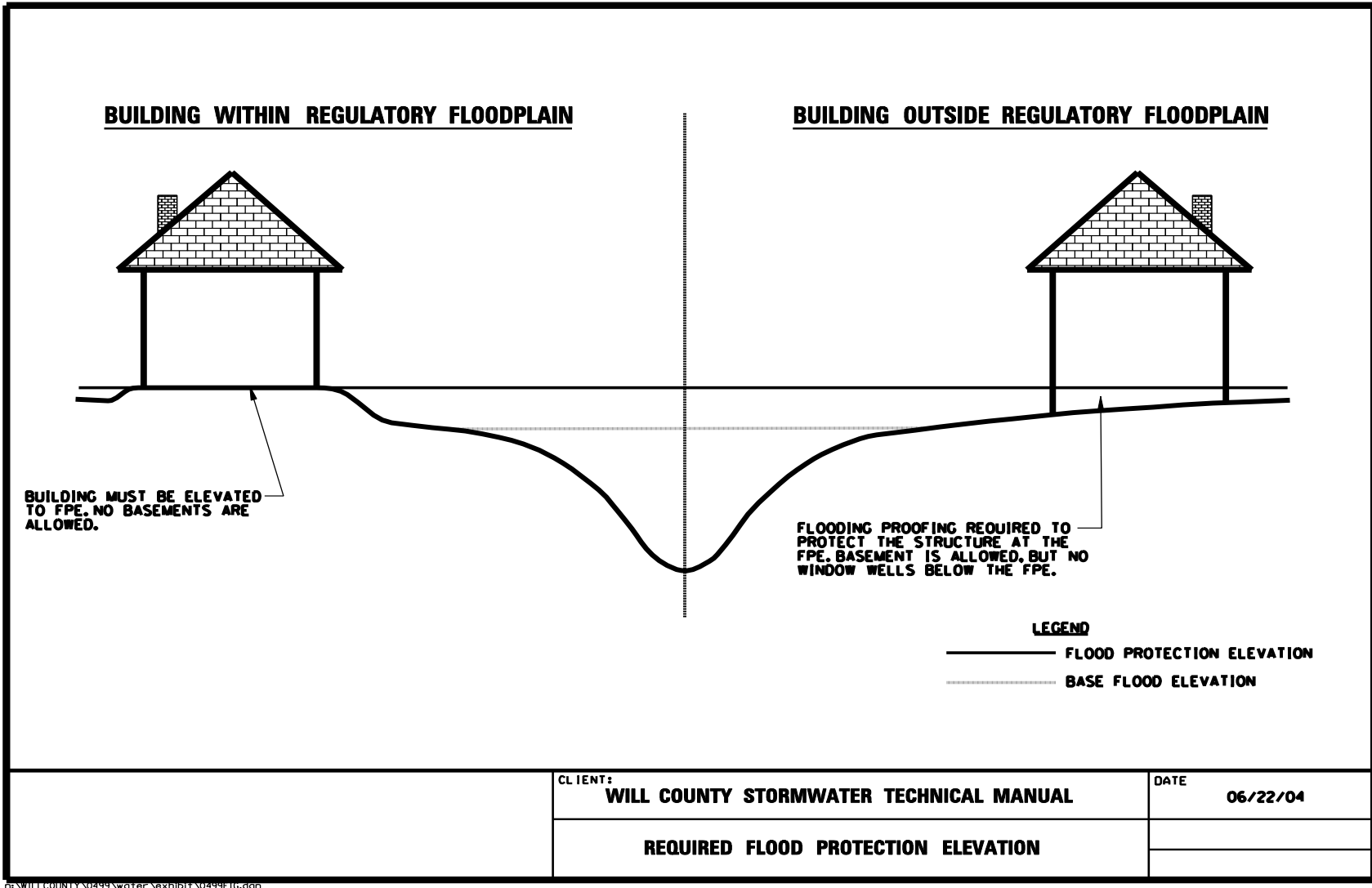
FIGURE 2 Required Flood Protection Elevation
