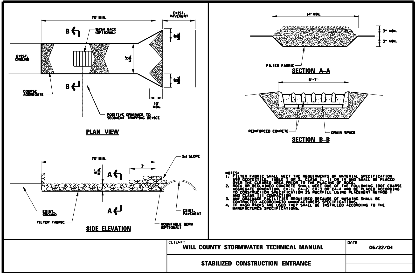
FIGURE 18 Stabilized Construction Entrance
