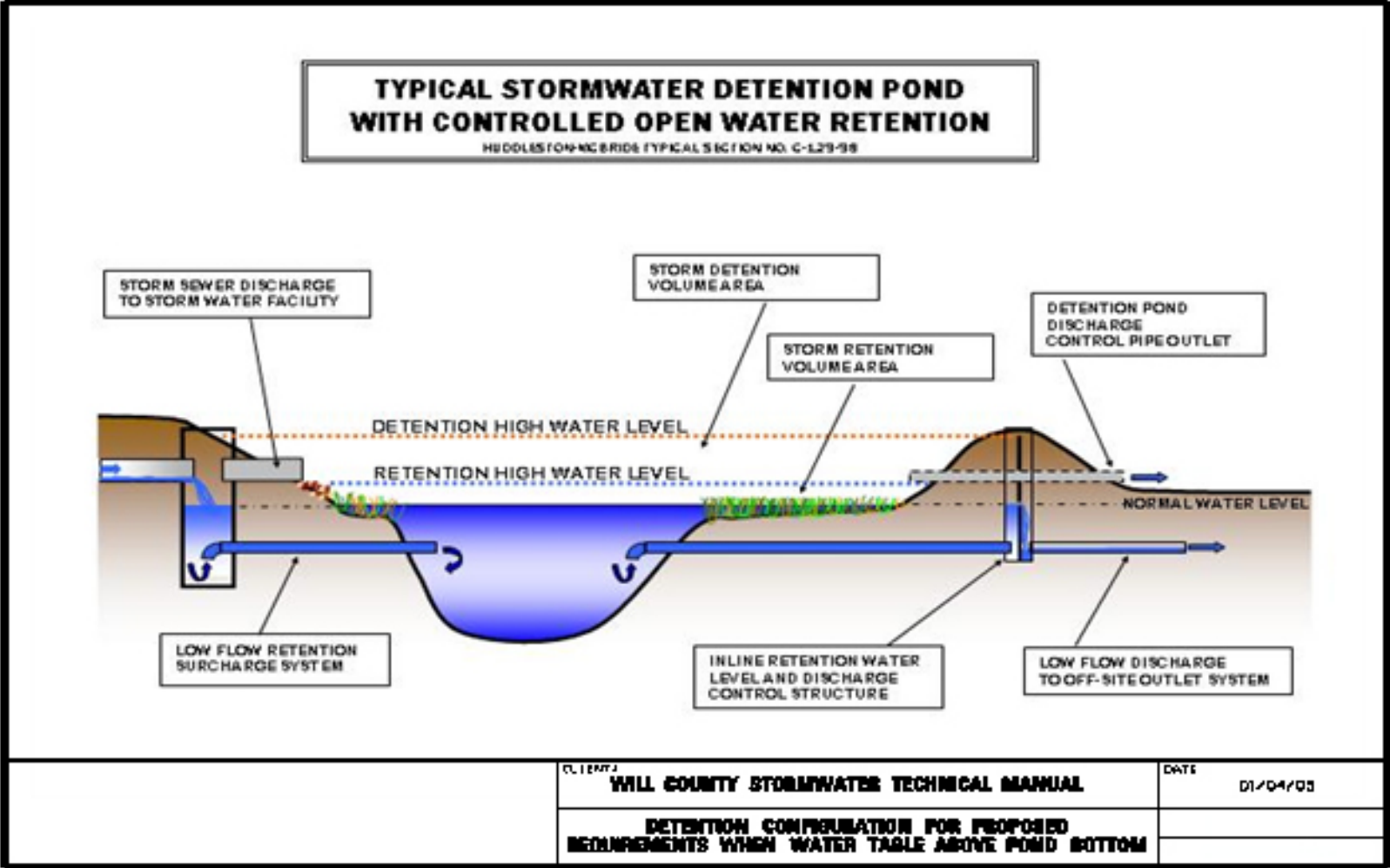
FIGURE 11 Detention Configuration for Proposed Requirements When Water Table is Above Pond Bottom
