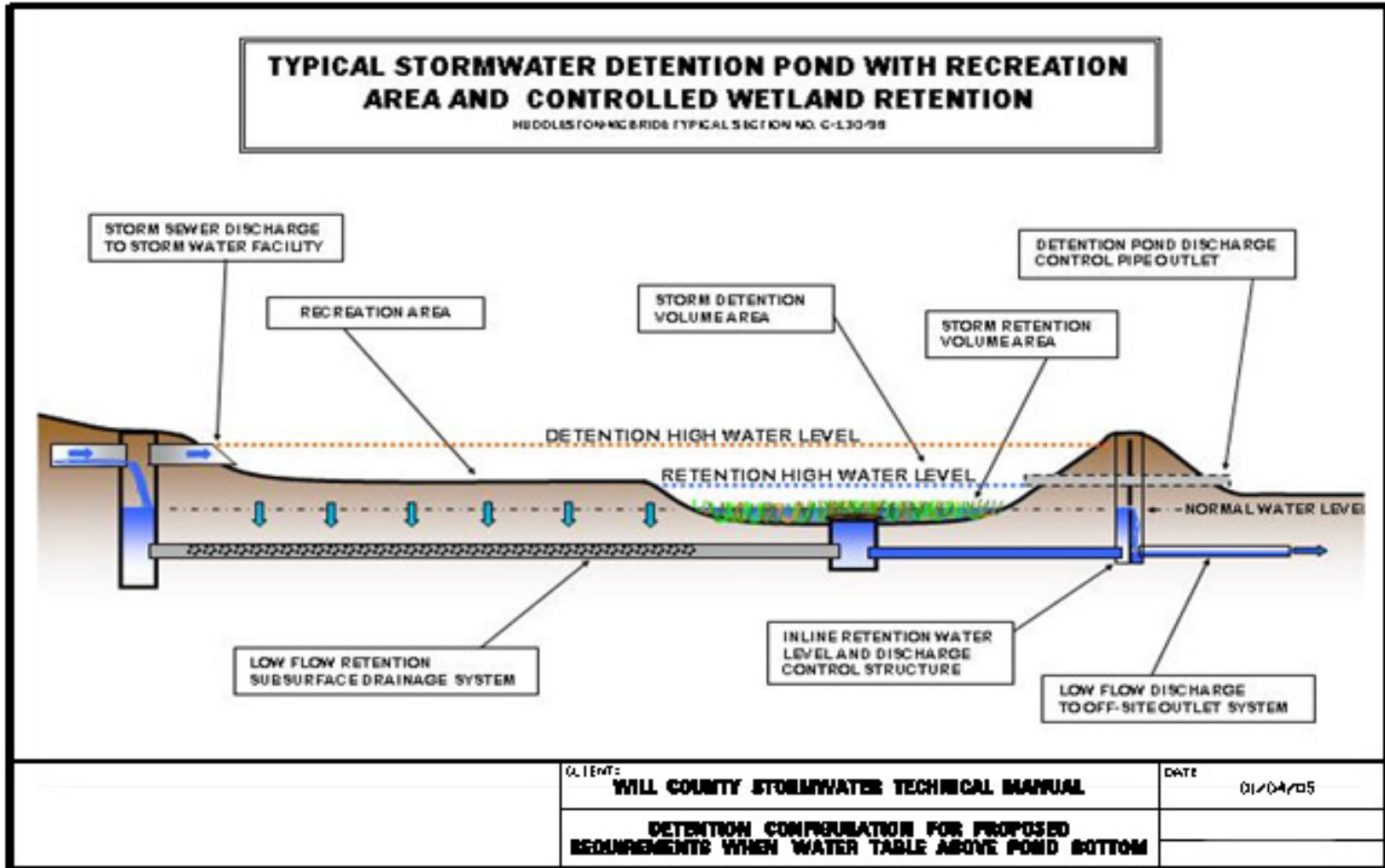
FIGURE 13 Detention Configuration for Proposed Requirements When Water Table is Above Pond Bottom
