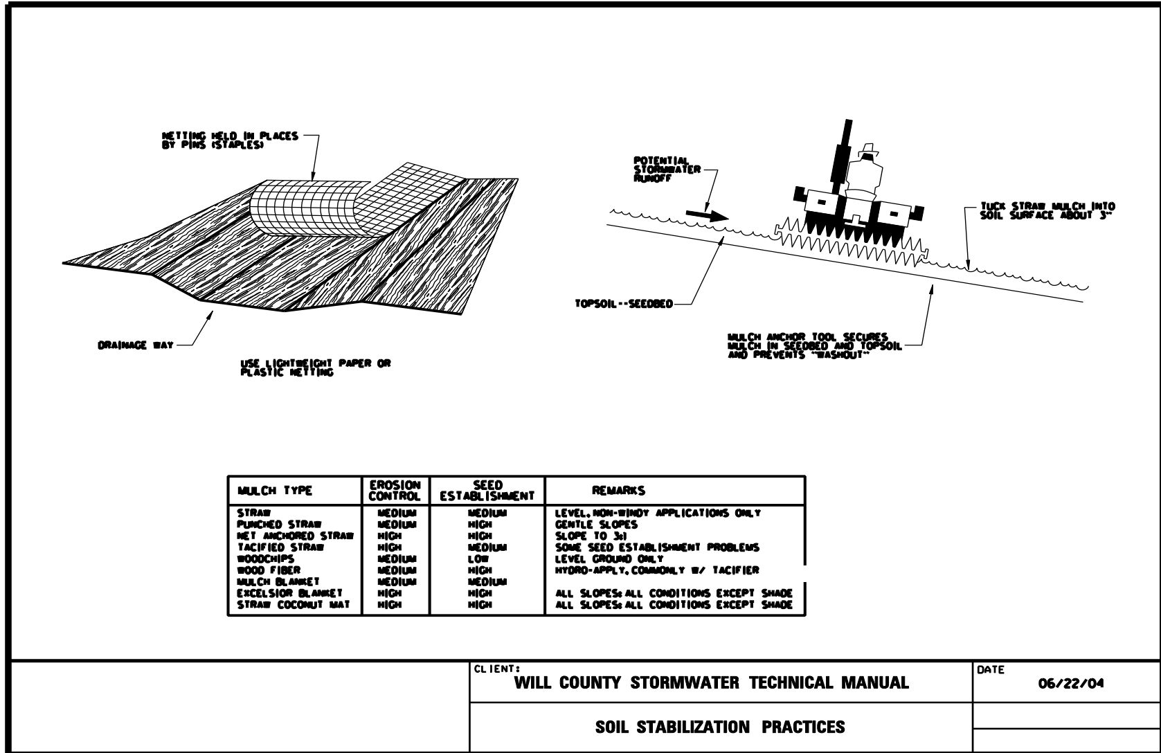
Figure 16A Soil Stabilization Practices
