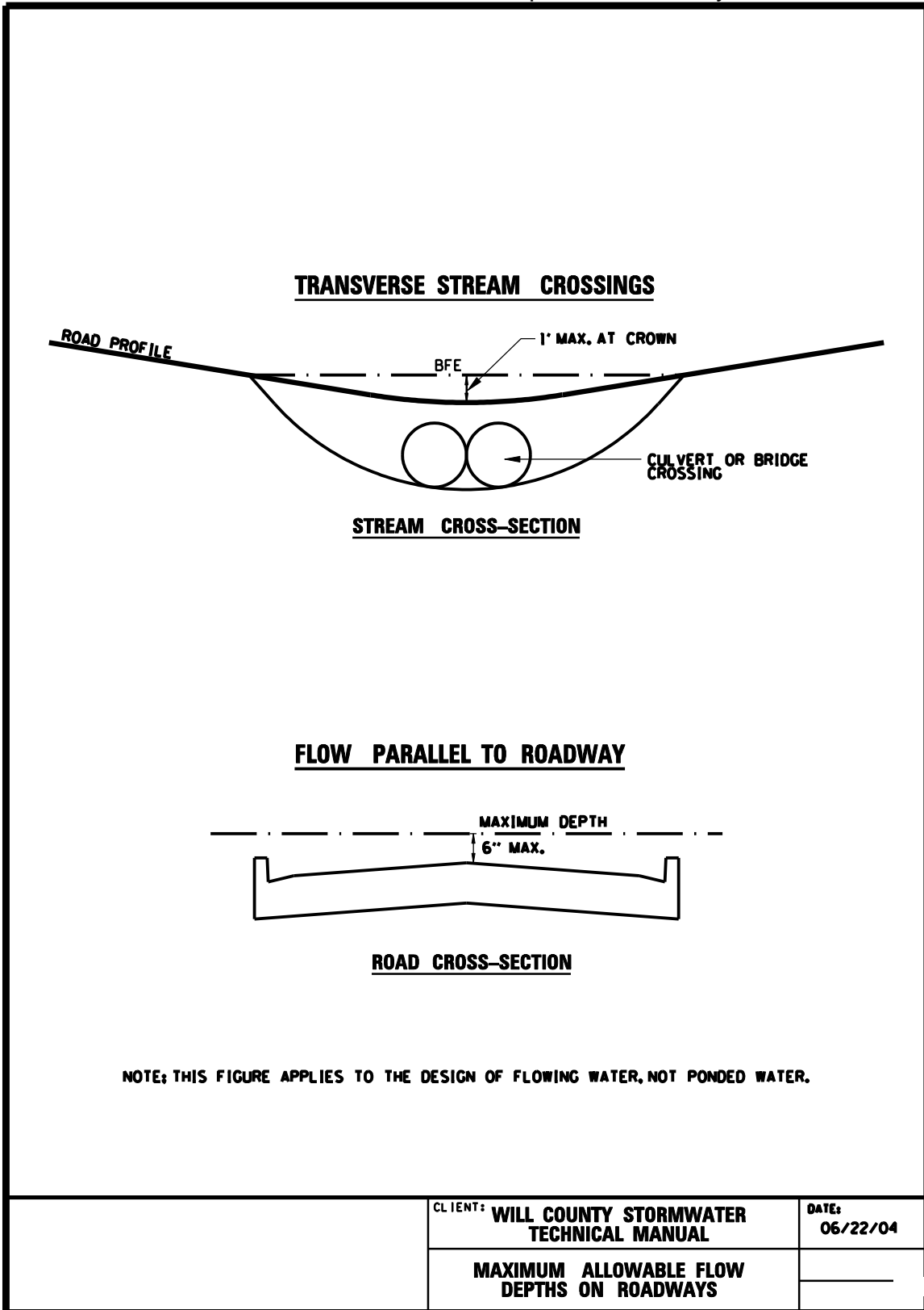
FIGURE 5 Maximum Allowable Flow Depths on Roadways
