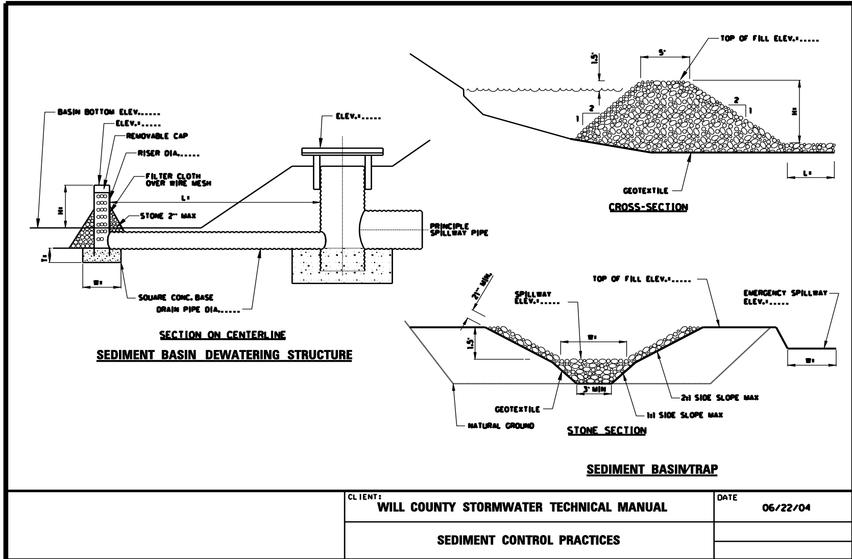
FIGURE 15A Sediment Control Practices
