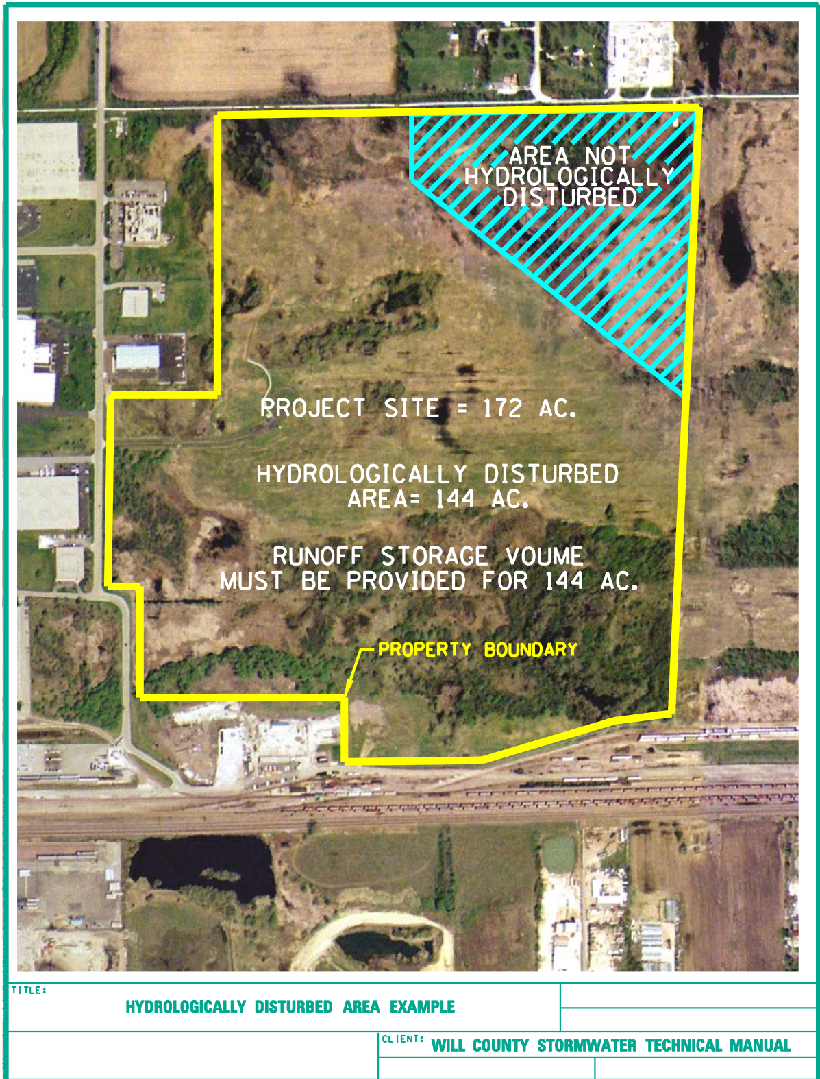
FIGURE 6 Hydrologically Disturbed Area Example
