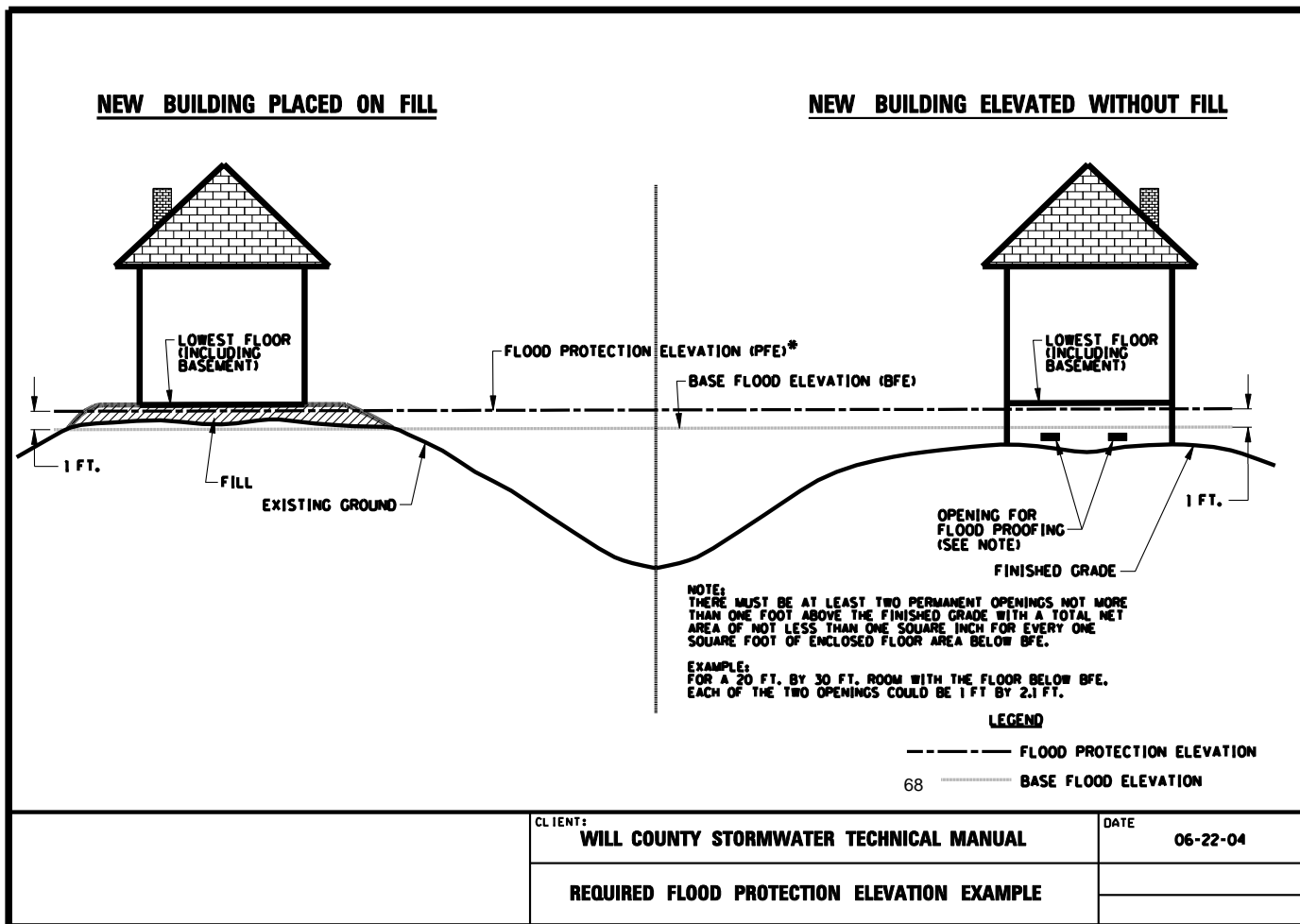
FIGURE 19 Required Flood Protection Elevation
