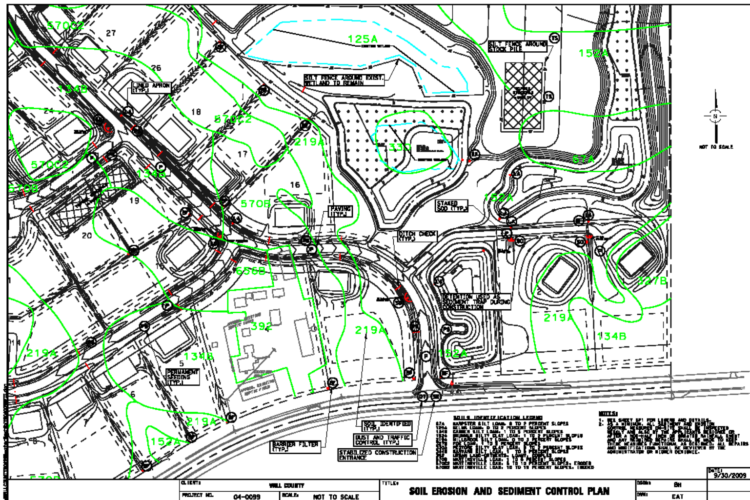
FIGURE 17 Sediment and Erosion Control Plan
