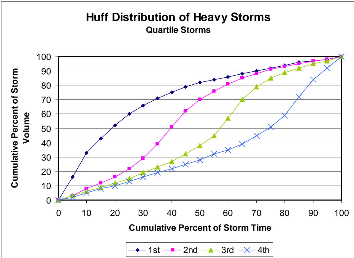
FIGURE 7 Median Time Distribution of Heavy Storm Rainfall at a Point (Reference: ISWS, 1992; Rainfall Frequency Atlas of the Midwest)
