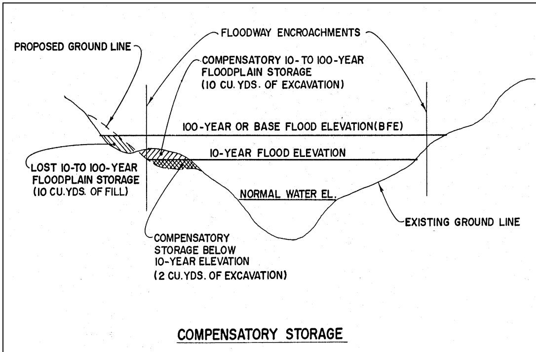
FIGURE 20 Compensatory Storage Example
