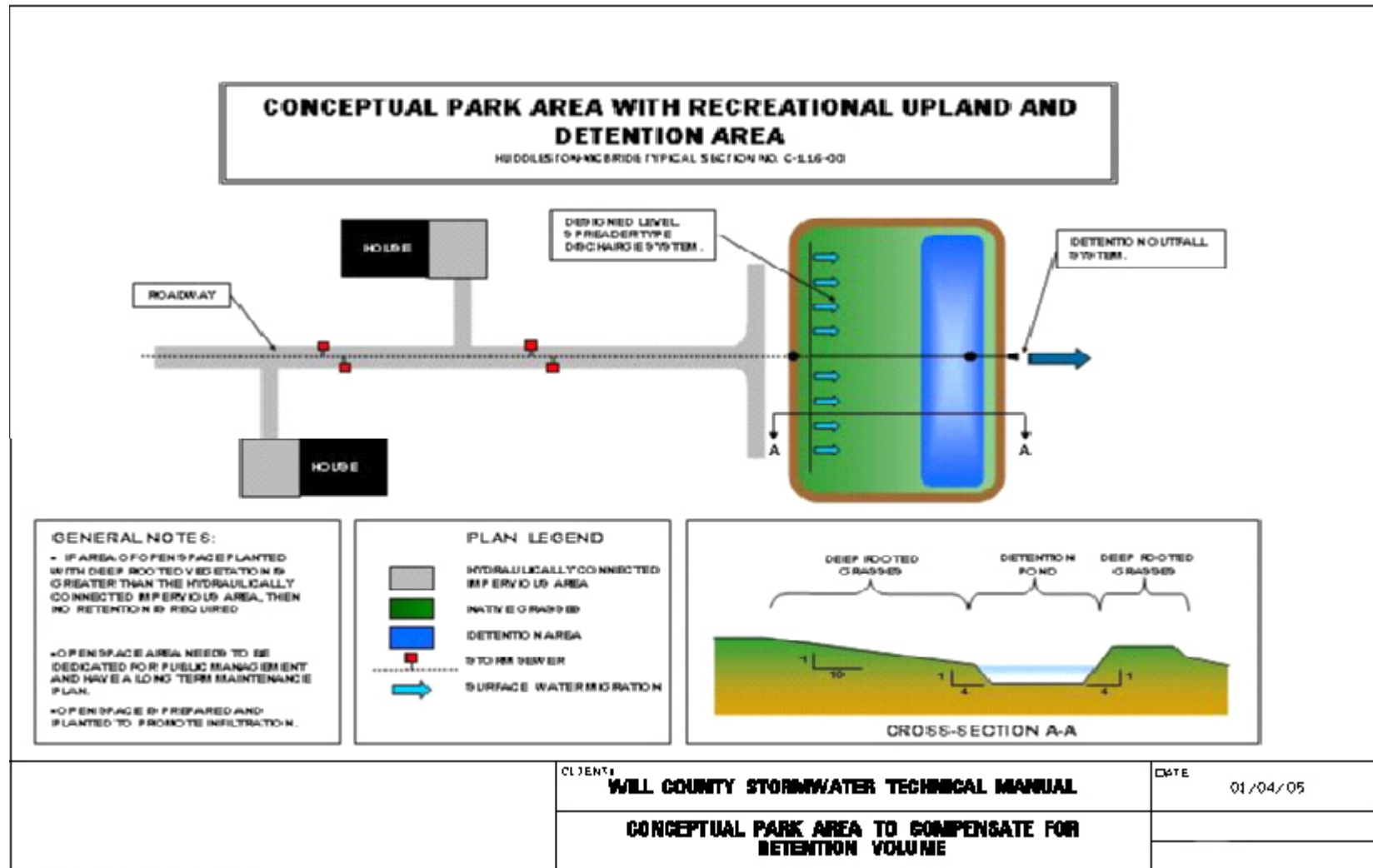
FIGURE 10 Conceptual Park Area to Compensate for Retention Volume
