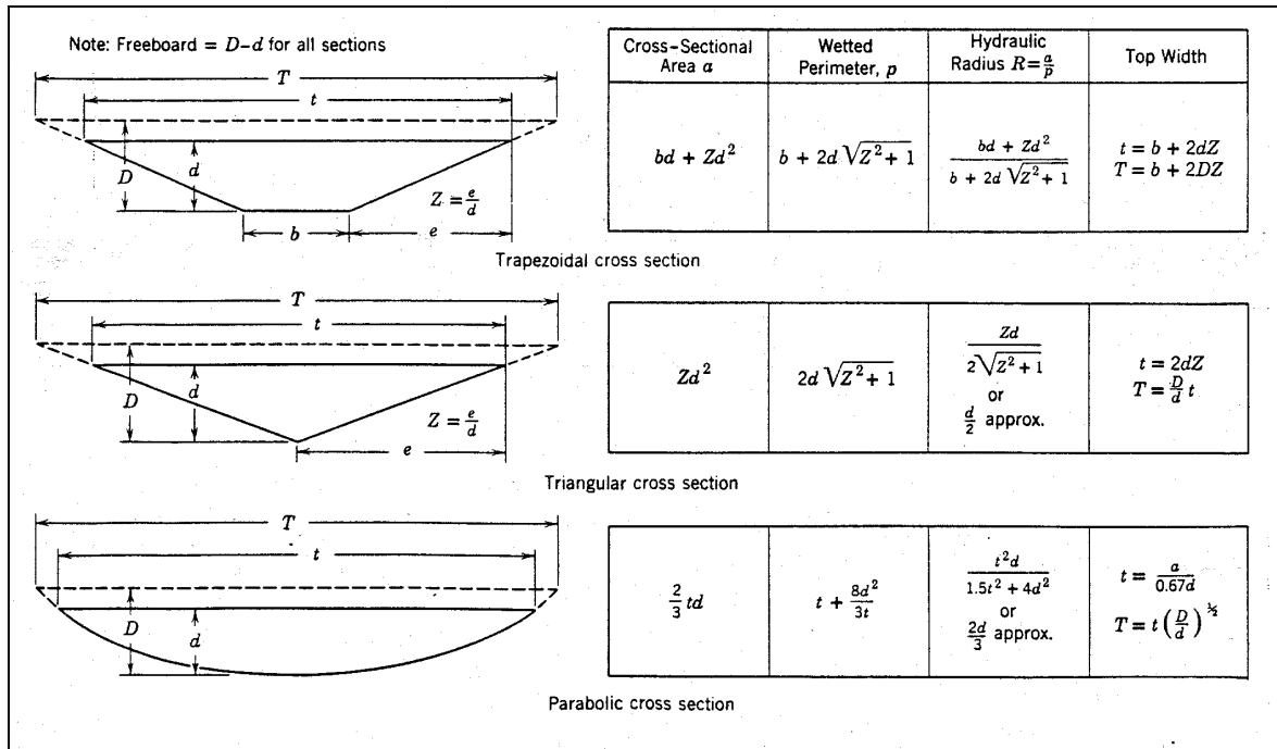
FIGURE 1 Geometric Elements of Channel Sections (Reference: Chow, Ven Te, 1959; Open-Channel Hydraulics)
