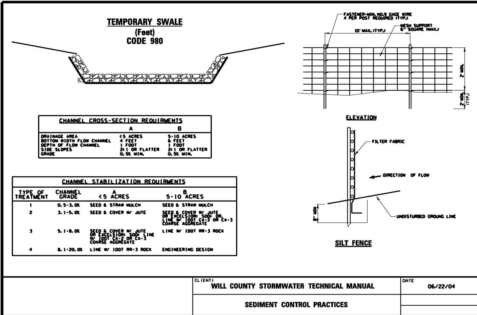
FIGURE 15B Sediment Control Practices
