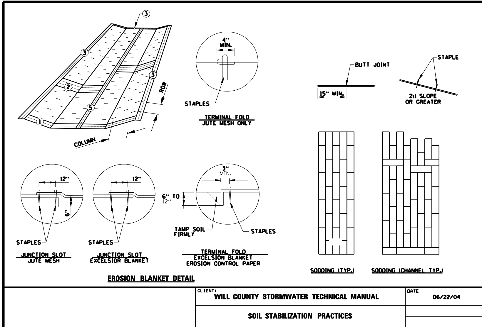
Figure 16B Soil Stabilization Practices
